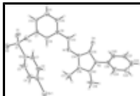
Fig. 1. The structure of (I), with displacement ellipsoids for non-H atoms drawn at the 30% probability level.
