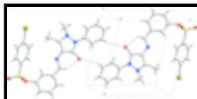
Fig. 2. A packing diagram for (I), with hydrogen bonds drawn as dashed lines.
